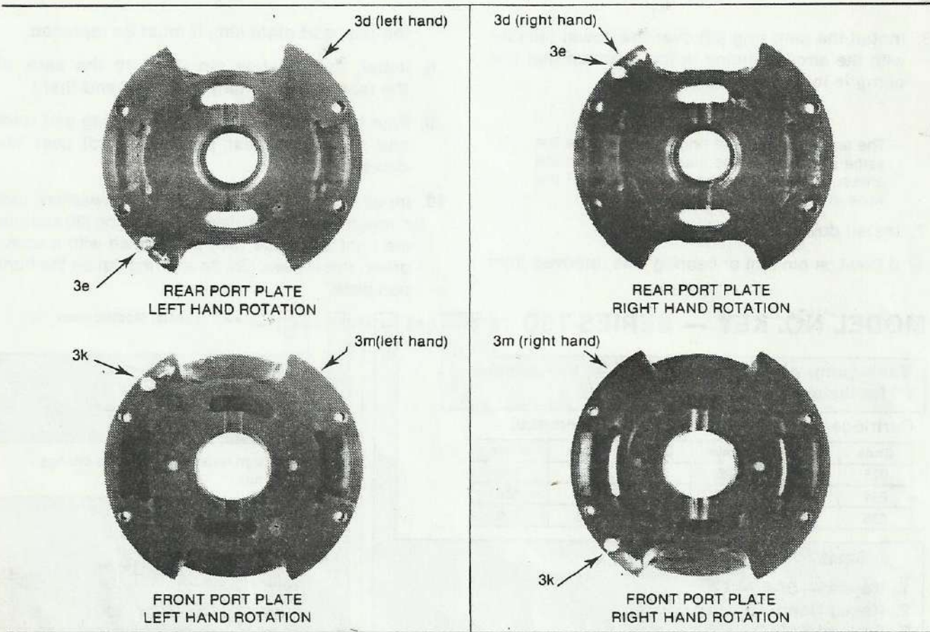
PUMP SHAFT ROTATION AS VIEWED FROM SHAFT END OF PUMP
