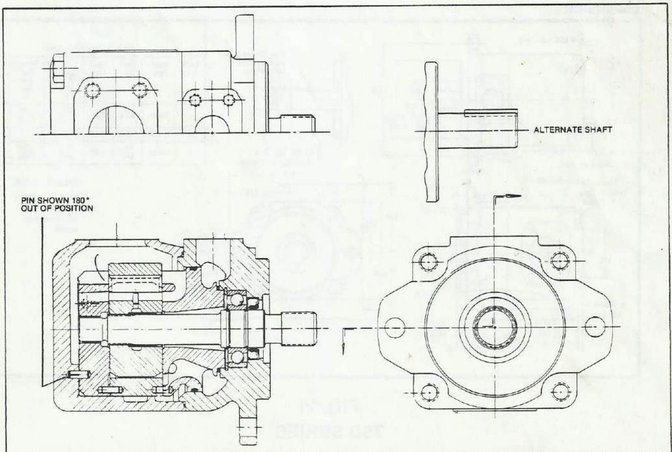
CROSS SECTION VIEW — T5D SERIES
